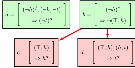
Figure 6.1: Defeasible normative reasoning examples: The Chisholm scenario (Example 6.1). Arrows denote defeat relations between arguments, relative to the constraint set \mathcal{C}' = \{-h^c\} (Example 6.2).
