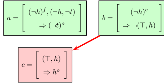
Figure 7.7: The contrary-to-duty scenario of Example 7.9.
