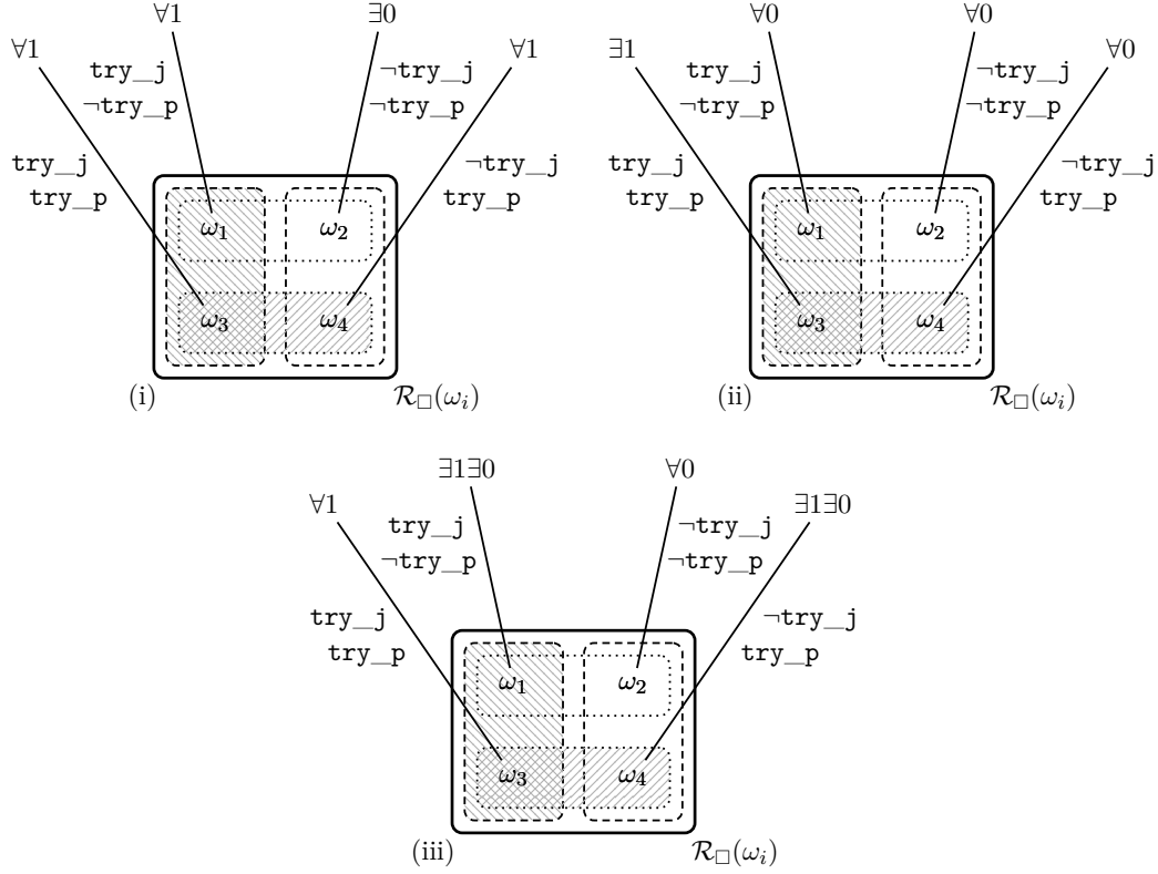
Figure 2.3: The only three scenarios (i)-(iii) for which [j]^d\text{try}_j and [p]^d\text{try}_p are satisfiable on a two-agent two-choice TUS n -model. \omega_i denotes an arbitrary non-empty set of worlds, for 1 \leq i \leq 4 . Choices of j are vertically presented, and those of p horizontally. The symbol \forall k at \omega_i with i \in \{1, 2, 3, 4\} means that every history h(\omega_i) is assigned value k , and \exists k at \omega_i means that some history h(\omega_i) going through the choice intersection is assigned k , for k \in \{0, 1\} . Deontically optimal choices are shaded and darker shaded when overlapping. At all \forall k outcomes with k \in \{0, 1\} , all obligations will be vacuously satisfied forever onward, and so CTD reasoning becomes impossible.
